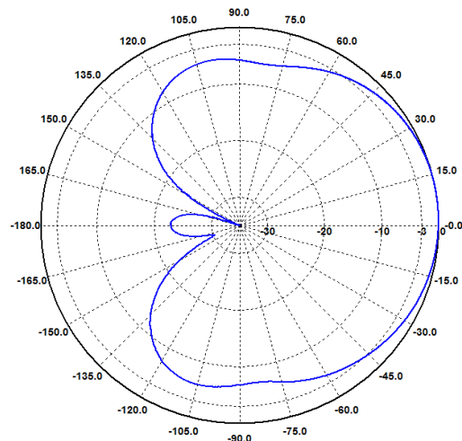
H-Ebene / H-Plane 500 MHz
