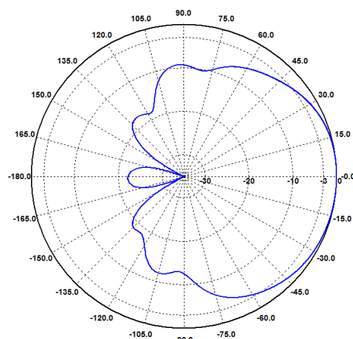
H-Ebene / H-Plane 900 MHz
