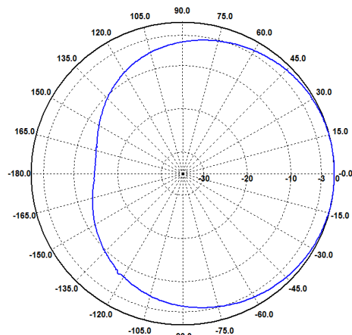
H-Ebene / H-Plane 300 MHz
