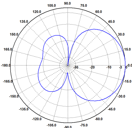
E-Ebene / E-Plane 400 MHz
