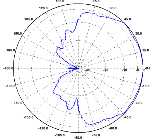
H-Ebene / H-Plane 3.0 GHz
