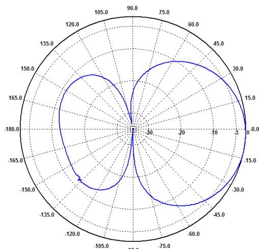
E-Ebene / E-Plane 300 MHz
