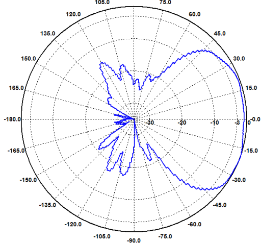
E-Ebene / E-Plane 3.0 GHz
