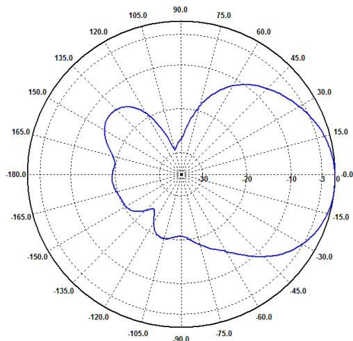
E-Ebene / E-Plane 500 MHz
