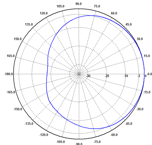
H-Ebene / H-Plane 400 MHz
